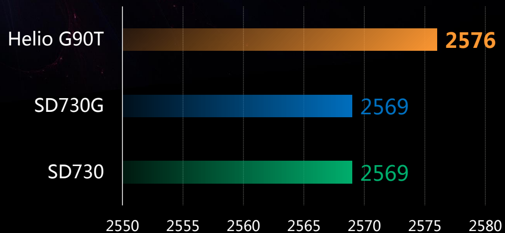
Geekbench - Single
