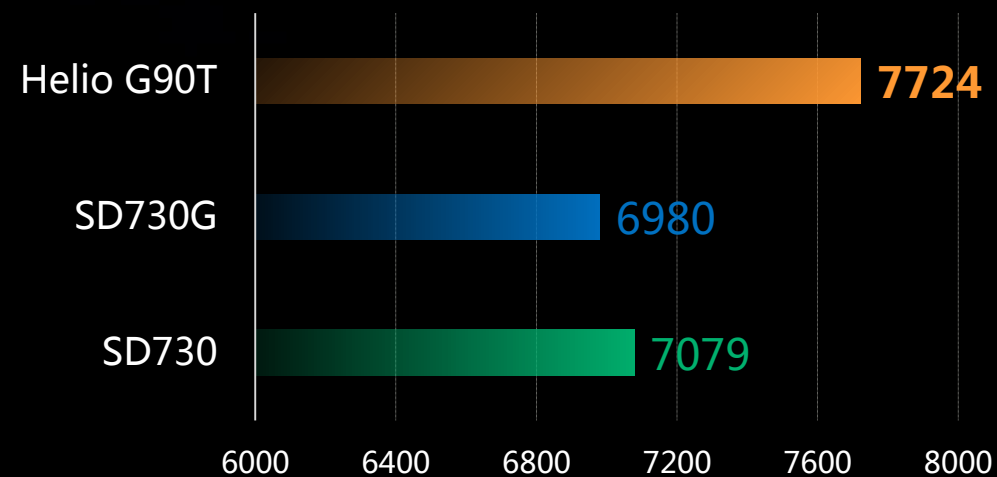
Geekbench - Multi
